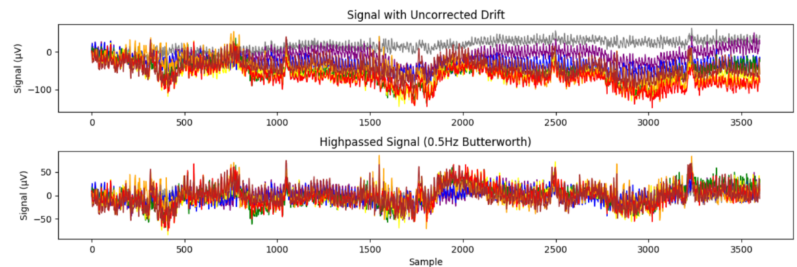
(a) DC offset and baseline drift were corrected using normalization and Butterworth high-pass ( \zeta 0.5 Hz) filter.
